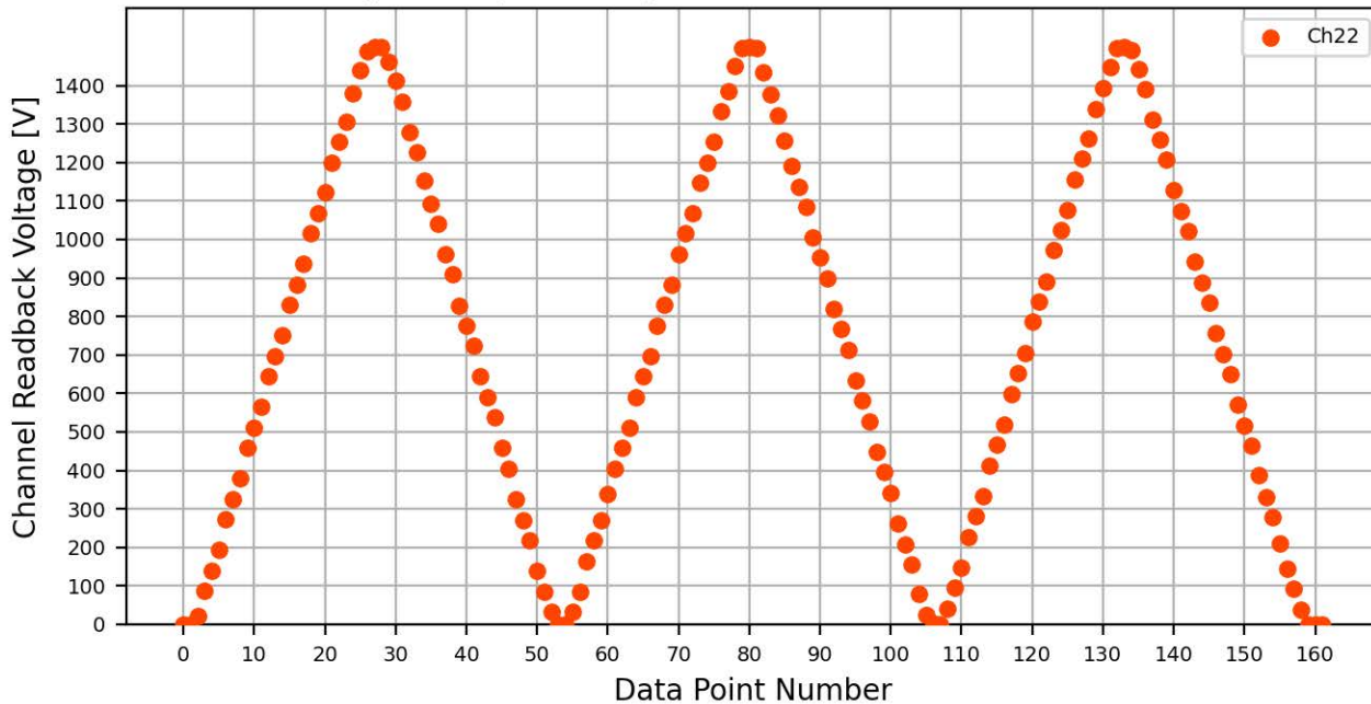
Voltage Ramp Test (Python) Bd #775, Slot #5, Ch #22
