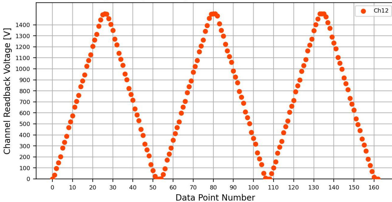
Voltage Ramp Test (Python) Bd #775, Slot #5, Ch #12
