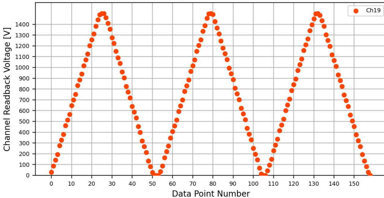
Voltage Ramp Test (Python) Bd #775, Slot #5, Ch #19
