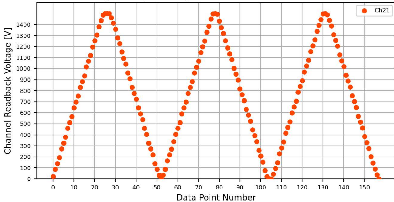
Voltage Ramp Test (Python) Bd #775, Slot #5, Ch #21
