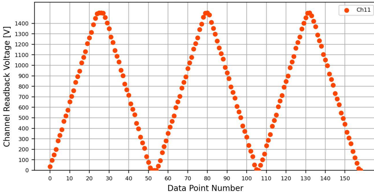
Voltage Ramp Test (Python) Bd #775, Slot #5, Ch #11
