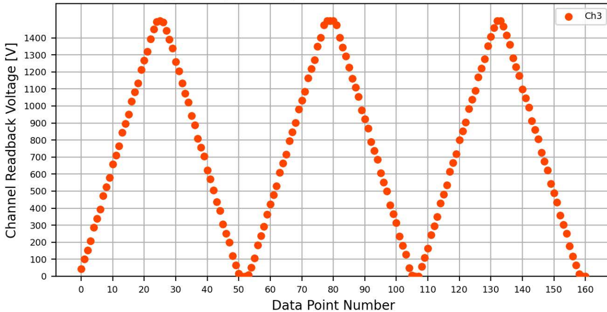
Voltage Ramp Test (Python) Bd #775, Slot #5, Ch #3
