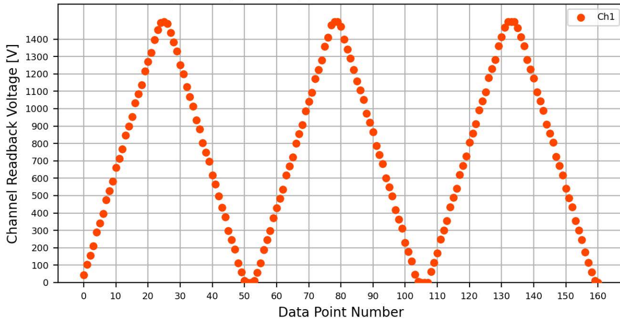
Voltage Ramp Test (Python) Bd #775, Slot #5, Ch #1
