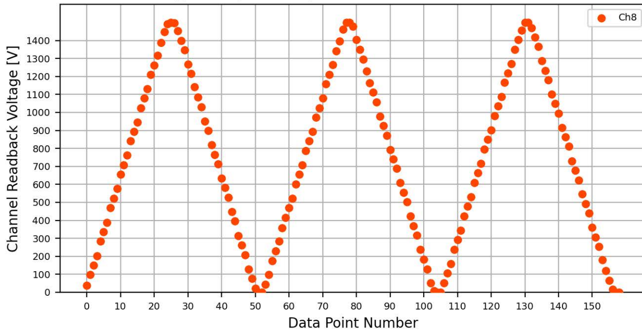
Voltage Ramp Test (Python) Bd #775, Slot #5, Ch #8
