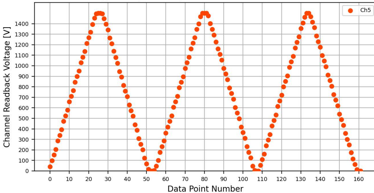
Voltage Ramp Test (Python) Bd #775, Slot #5, Ch #5
