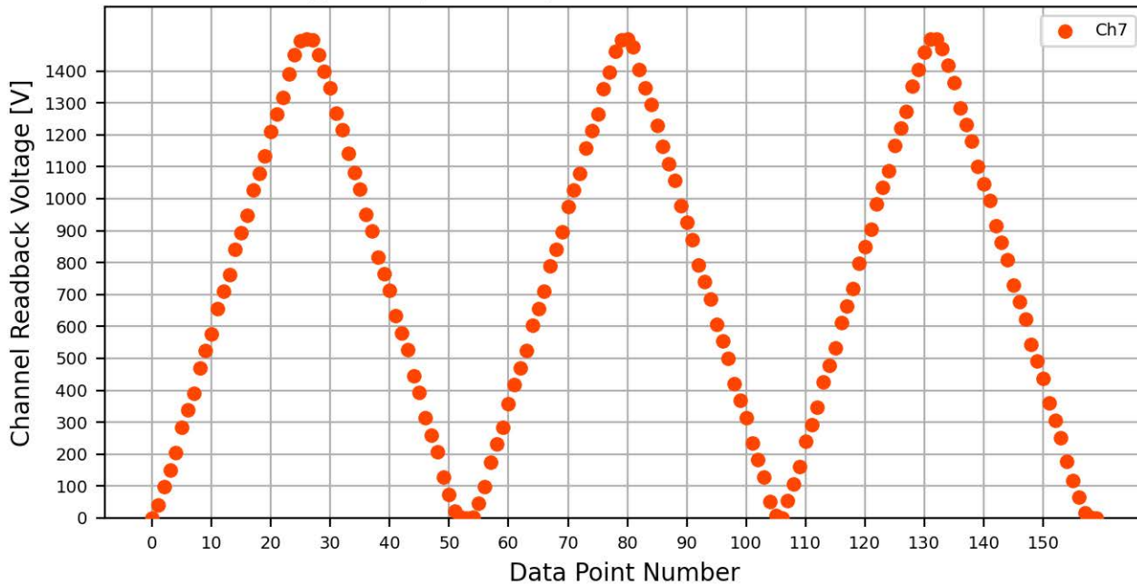
Voltage Ramp Test (Python) Bd #775, Slot #5, Ch #7
