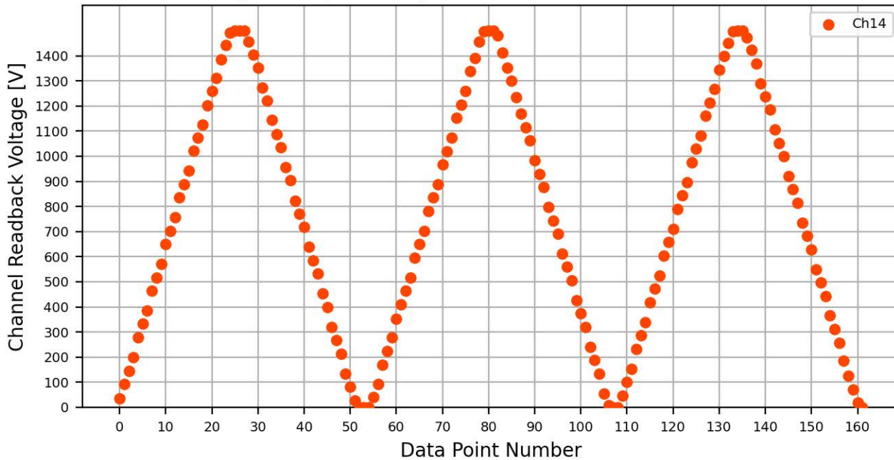
Voltage Ramp Test (Python) Bd #775, Slot #5, Ch #14
