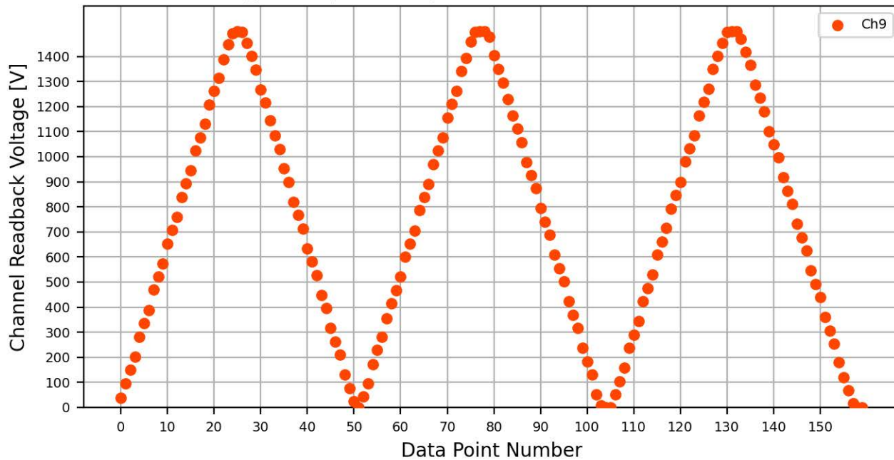
Voltage Ramp Test (Python) Bd #775, Slot #5, Ch #9
