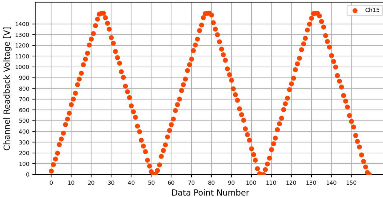
Voltage Ramp Test (Python) Bd #775, Slot #5, Ch #15
