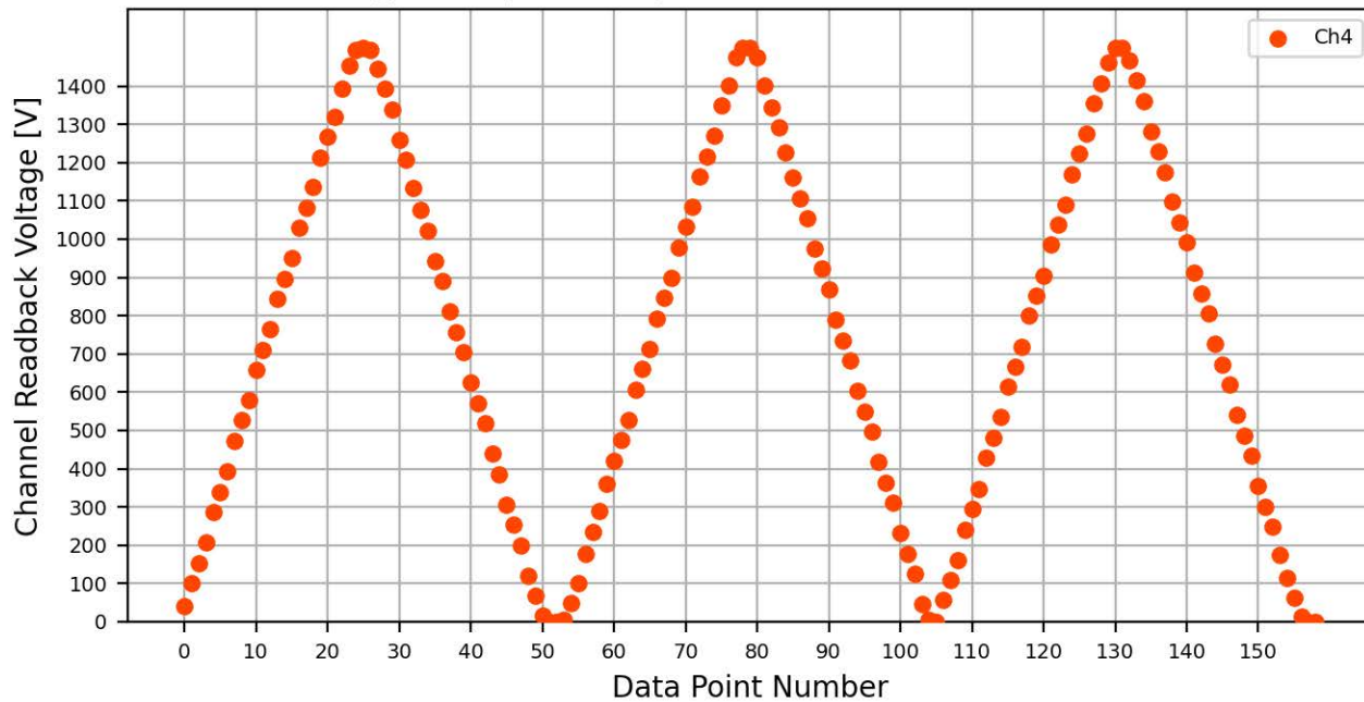
Voltage Ramp Test (Python) Bd #775, Slot #5, Ch #4
