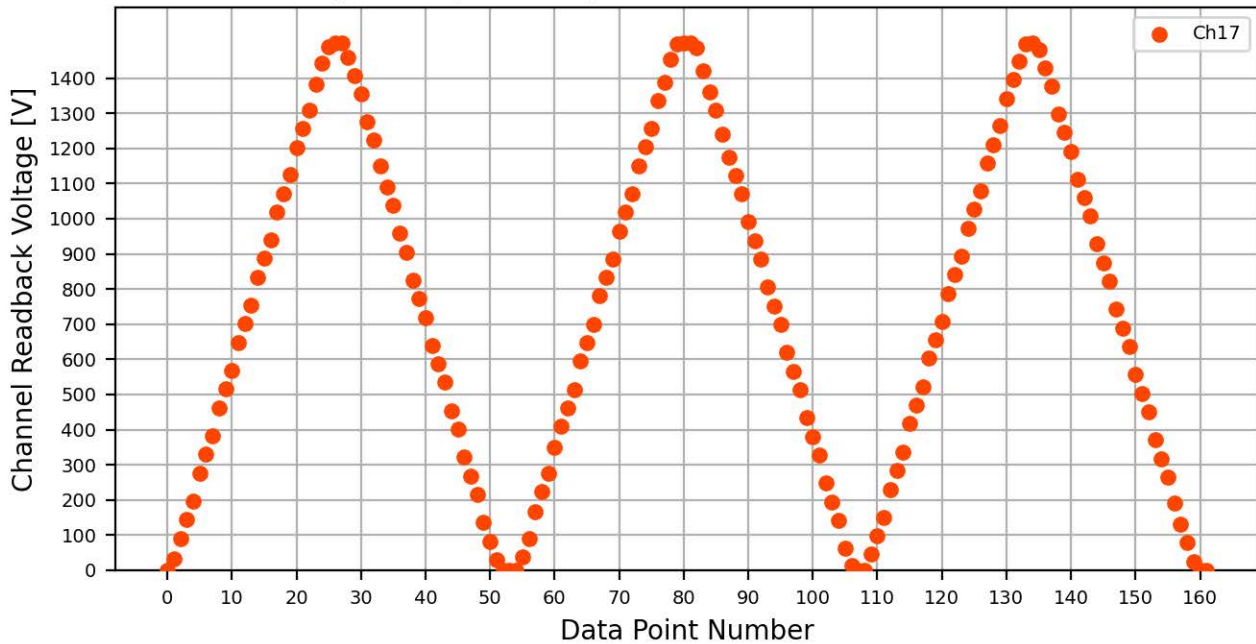
Voltage Ramp Test (Python) Bd #775, Slot #5, Ch #17
