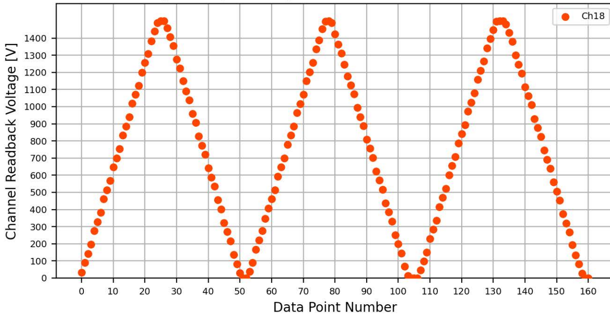
Voltage Ramp Test (Python) Bd #775, Slot #5, Ch #18
