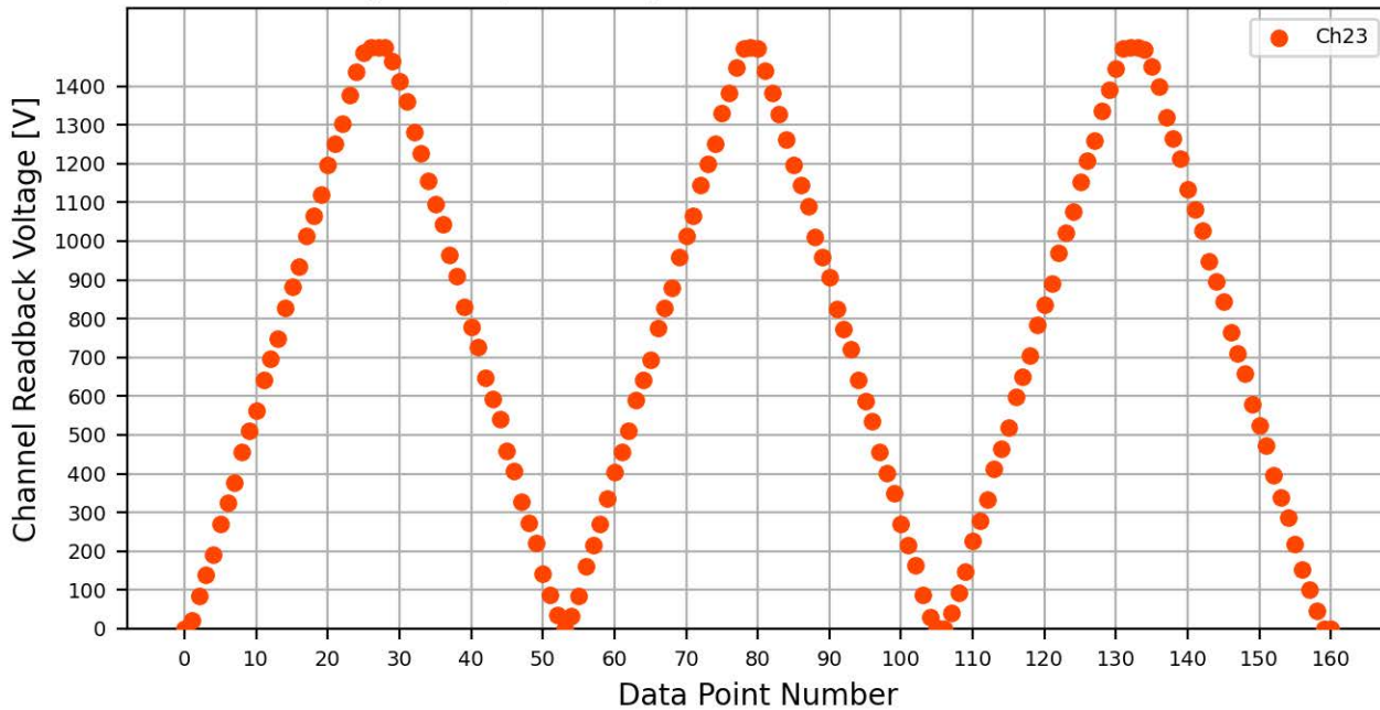
Voltage Ramp Test (Python) Bd #775, Slot #5, Ch #23
