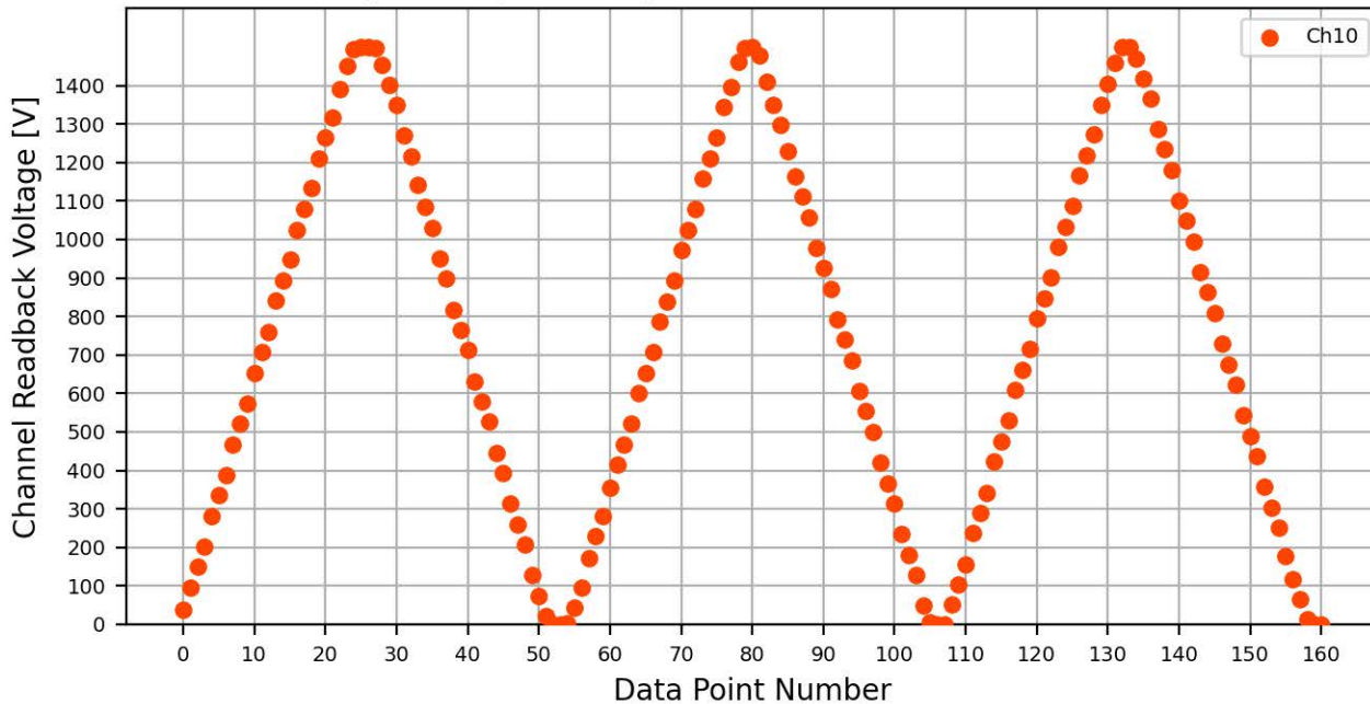
Voltage Ramp Test (Python) Bd #775, Slot #5, Ch #10
