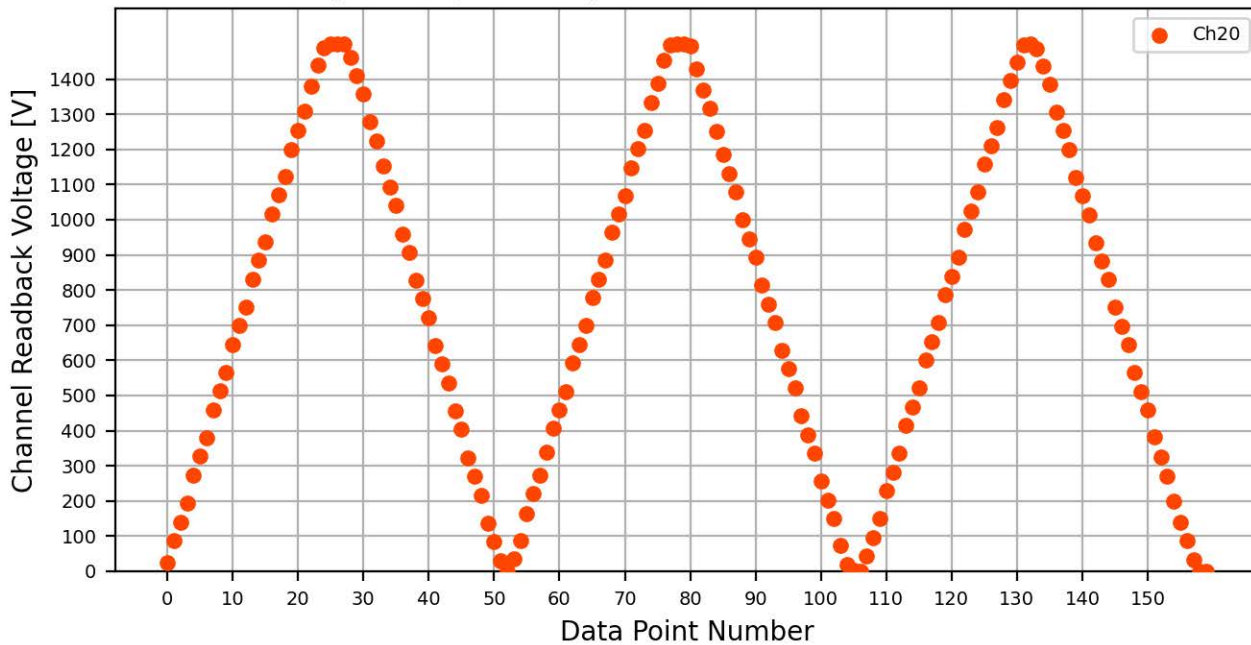
Voltage Ramp Test (Python) Bd #775, Slot #5, Ch #20
