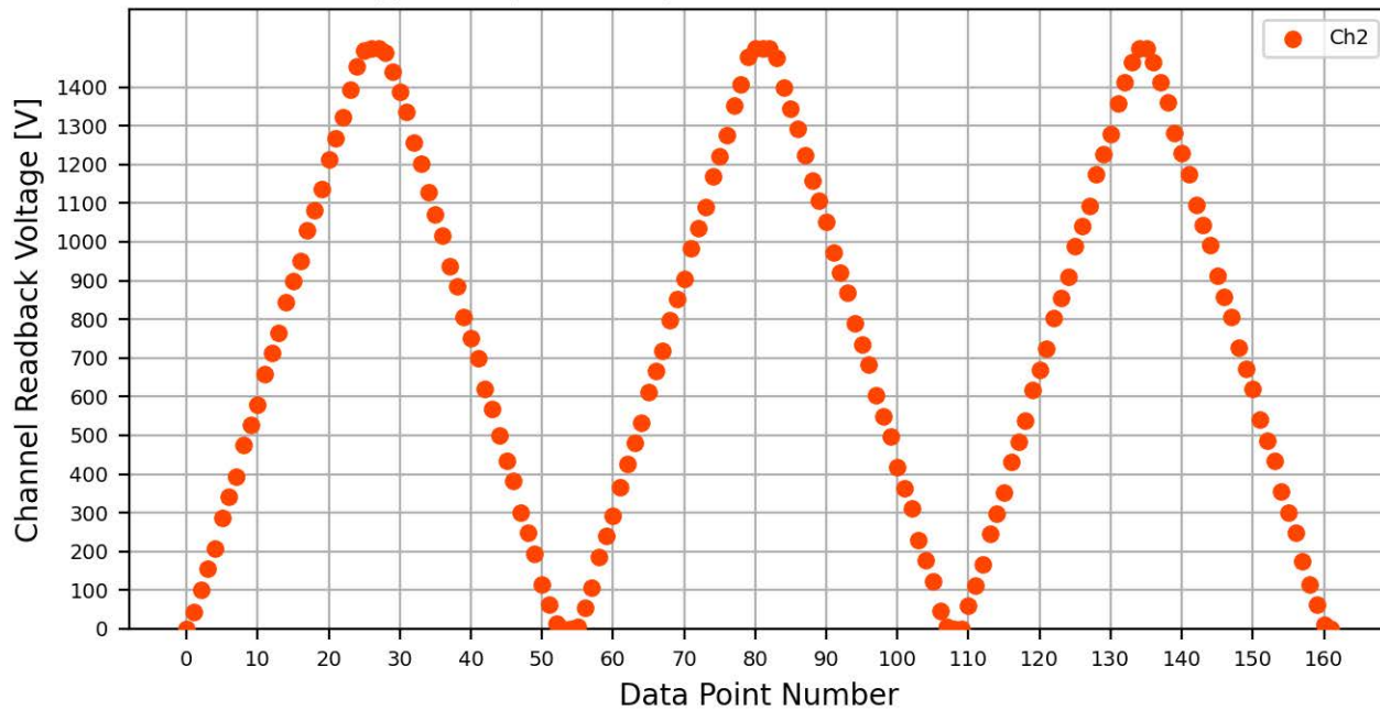
Voltage Ramp Test (Python) Bd #775, Slot #5, Ch #2
