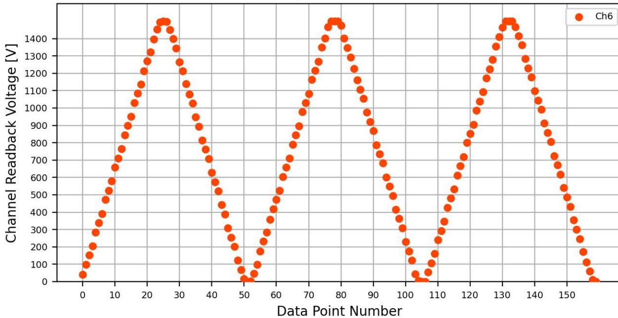
Voltage Ramp Test (Python) Bd #775, Slot #5, Ch #6
