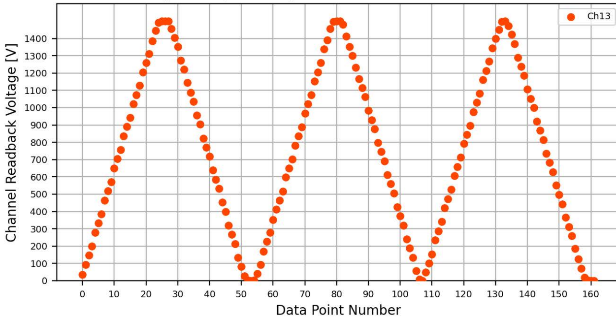
Voltage Ramp Test (Python) Bd #775, Slot #5, Ch #13
