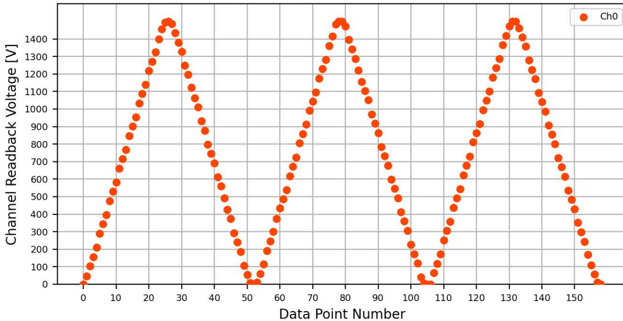
Voltage Ramp Test (Python) Bd #775, Slot #5, Ch #0
